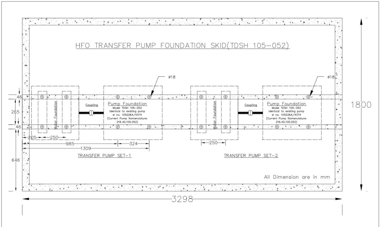
Figure-4: Skid Foundation (Item No.:2)
