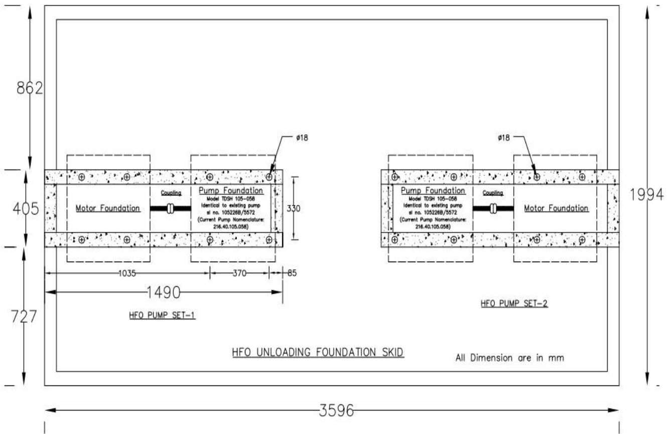
Figure-2: Skid Foundation (Item No.:1)
