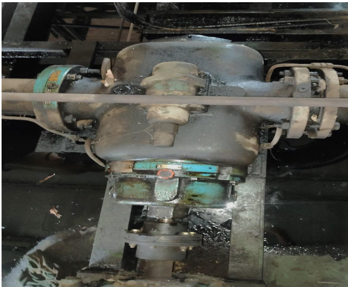
Figure-3: Sample Picture of Horizontal Twin Screw Pump (Item No.:1)
